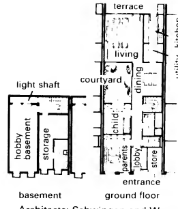
③ 180 m² living area
